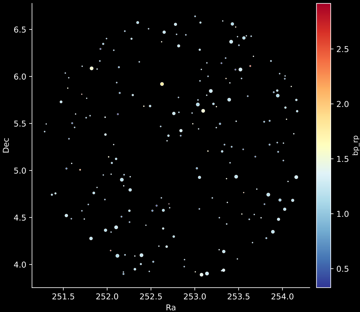
APOGEE DR17 Field: [235+46_MGA] Stars: 207
