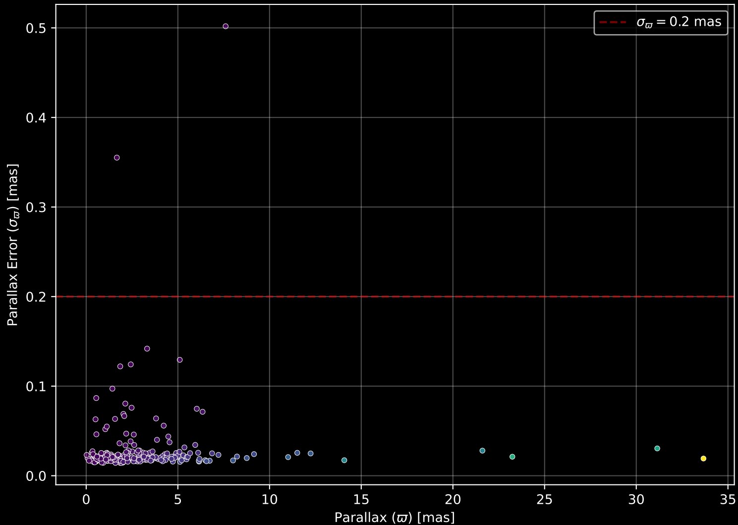
APOGEE DR17 Field: [235+46_MGA] Parallax Quality (n= 207)
