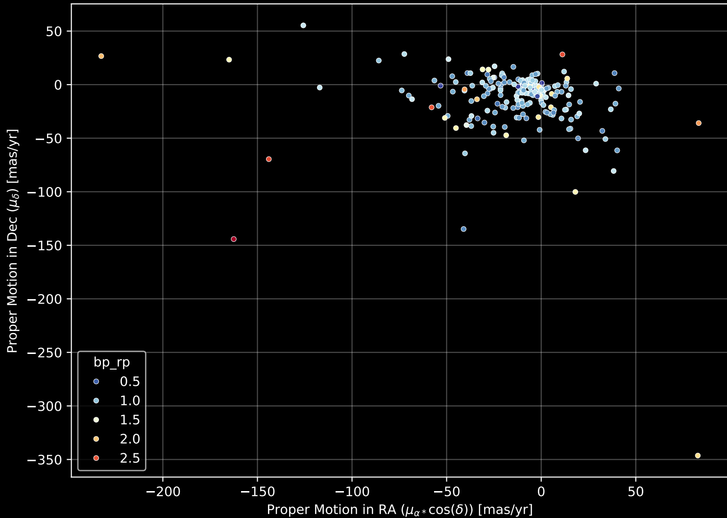
APOGEE DR17 Field: [235+46_MGA] Proper Motion Diagram (n= 207)
