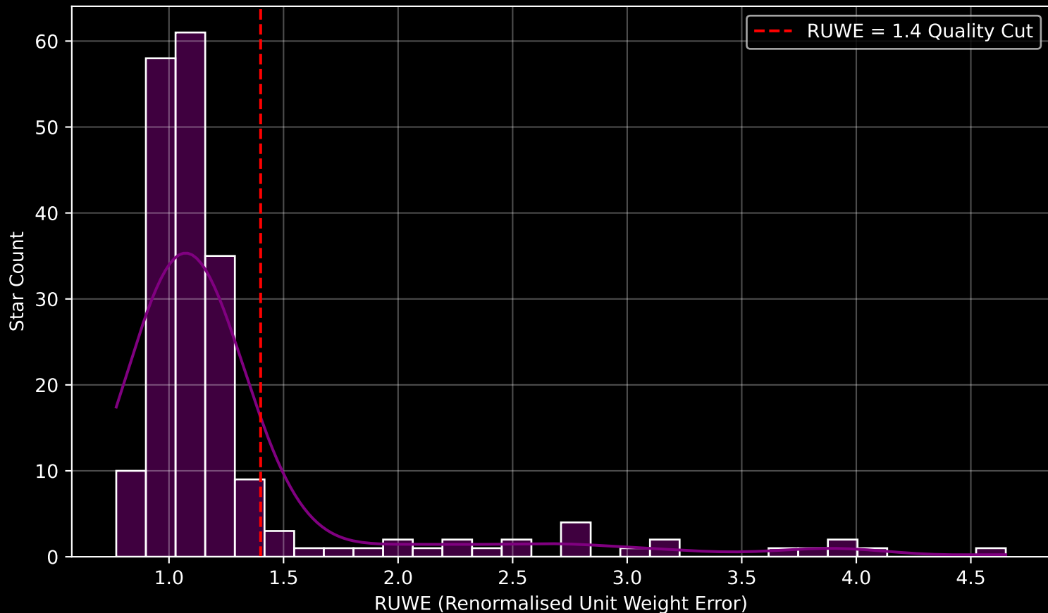
GAPOGEE DR17 Field [235+46_MGA] RUWE Distribution (n= 200)
