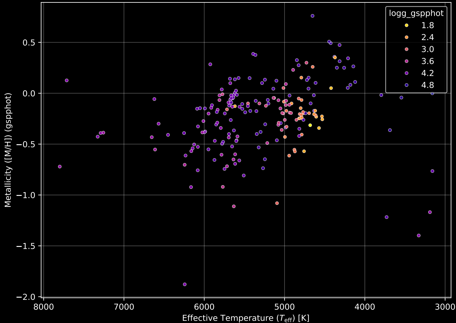
APOGEE DR17 Field: [235+46_MGA] Stellar Population Parameters (n= 207)
