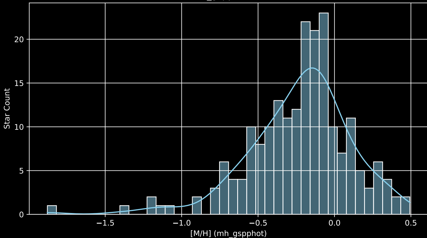
APOGEE DR17 Field: [235+46_MGA [M/H] (mh_gspphot) (n= 205)
