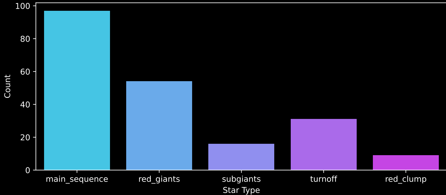
APOGEE DR17 Field: [235+46_MGA] Count plot of Star Type
